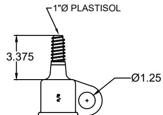
END FITTING VIEW - P-6511-01E
